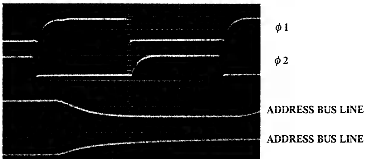
FIGURE 3.7b – Excess Address Line Loading
